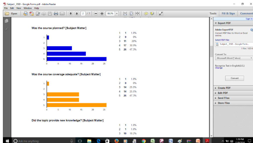
Fig. 4: Sample Analysis
