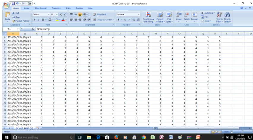
Fig. 3: Sample Responses
